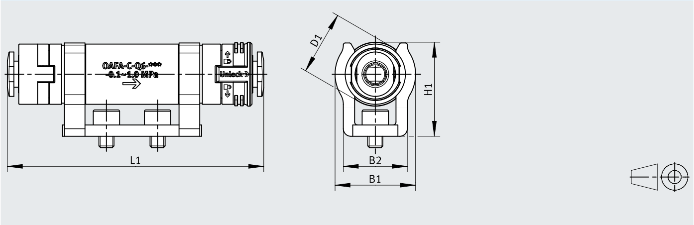
Dimensions – Inline filter OAFA
