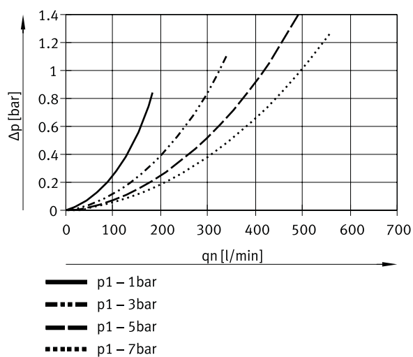
Normal flow rate q_n as a function of differential pressure \Delta p (OAFA-C-Q6-E-F)
