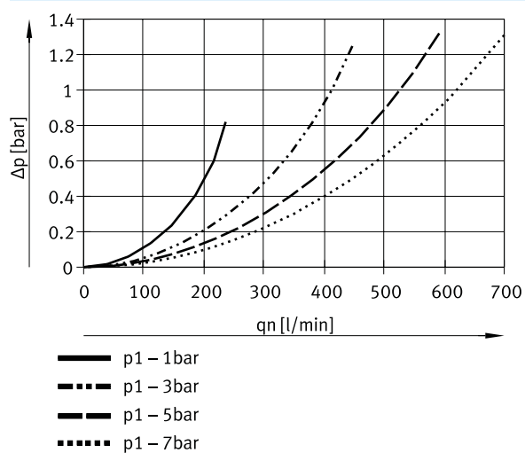
Normal flow rate q_n as a function of differential pressure \Delta p (OAFA-C-Q6-E-E)
