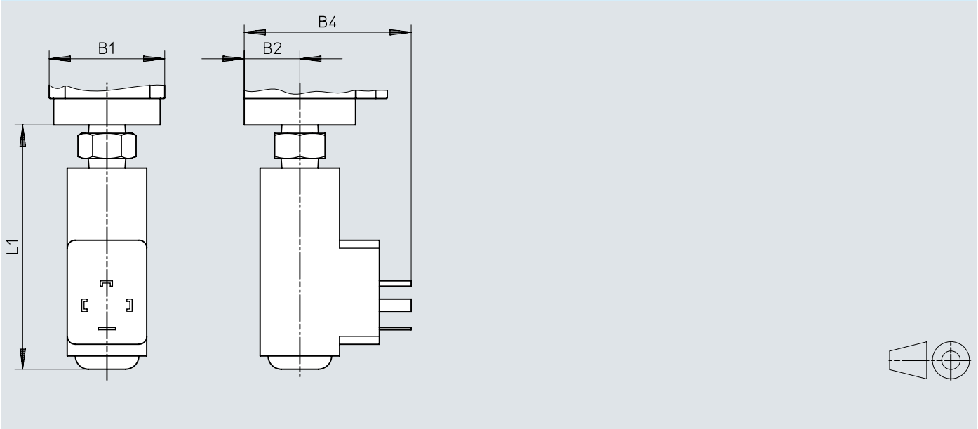
Dimensions – X/Y pressure switch with adjustable pressure switch point
