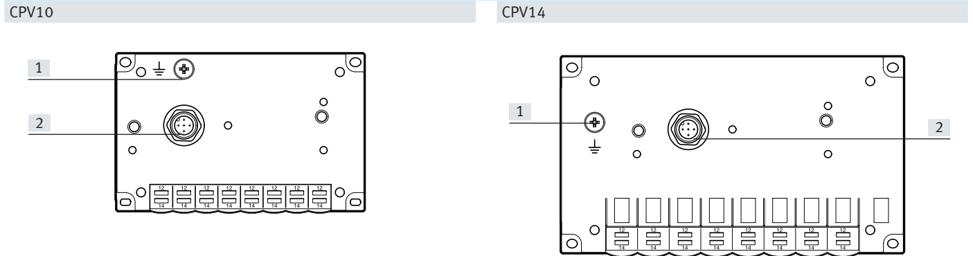
[1] Earthing screw [2] I-Port interface/IO-Link® [1] Earthing screw [2] I-Port interface/IO-Link®
