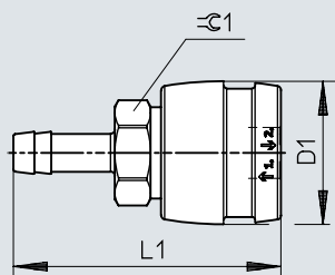
Dimensions – Coupling socket for plug-in nipple
