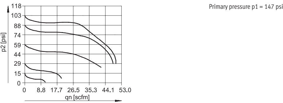
Normal flow qn as a function of output pressure p2 (MSB4N-1/8; pressure regulation range 7.4 ... 176 psi; grade of filtration 5 µm)
