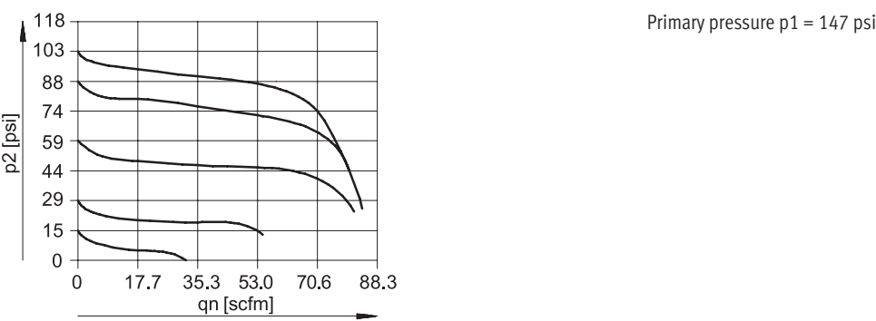
Normal flow qn as a function of output pressure p2 (MSB4N-1/4; pressure regulation range 4.4 ... 103 psi; grade of filtration 5 µm)
