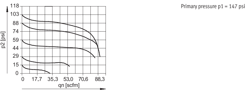
Normal flow qn as a function of output pressure p2 (MSB4N-1/4; pressure regulation range 4.4 ... 103 psi; grade of filtration 40 µm)
