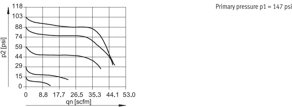
Normal flow qn as a function of output pressure p2 (MSB4N-1/8; pressure regulation range 7.4 ... 176 psi; grade of filtration 40 µm)
