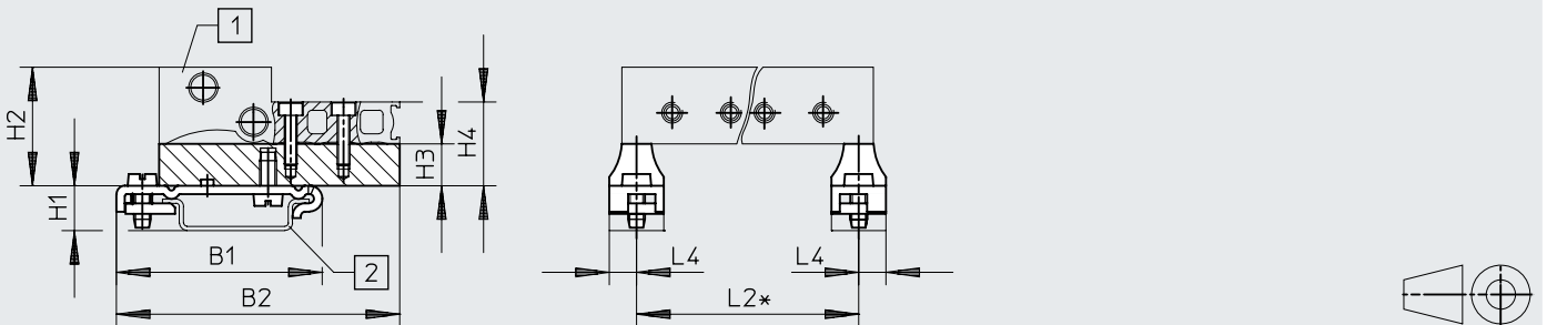
[1] Manifold block
