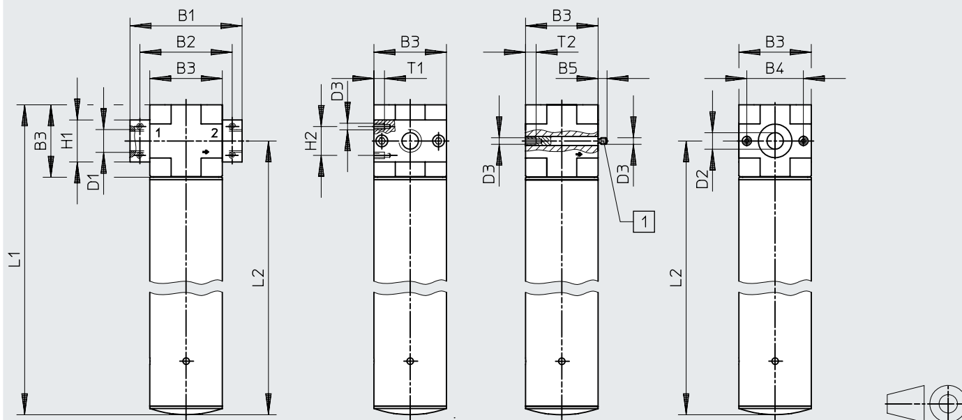
Dimensions – Membrane air dryer LDM1
