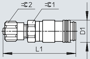
Dimensions – Coupling socket KD3, quick connector
