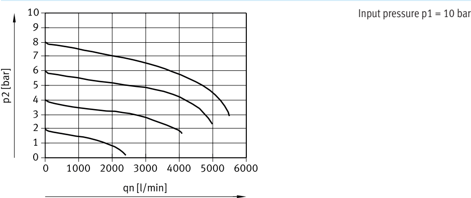
Standard flow rate qn as a function of output pressure p2 (FRC/FRCS-1/2-D-MIDI)
