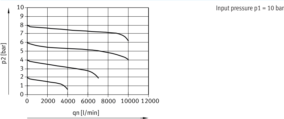
Standard flow rate qn as a function of output pressure p2 (FRC-1-D-MAXI)
