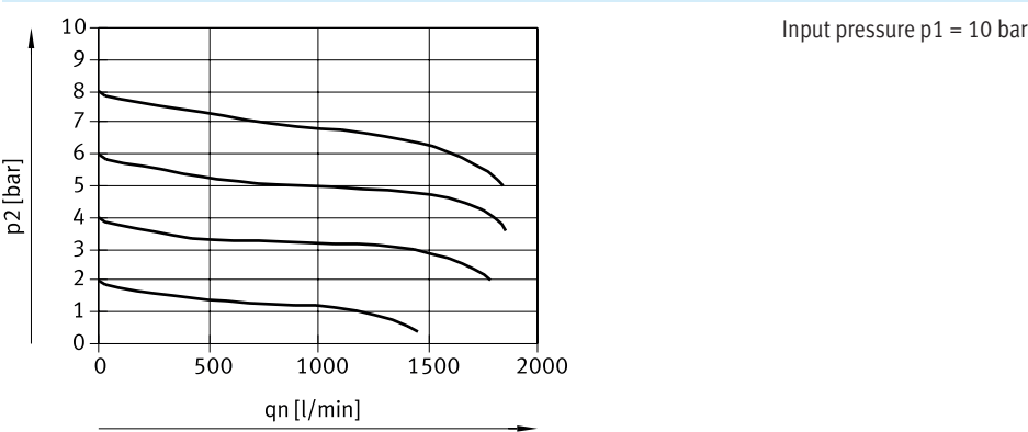
Standard flow rate qn as a function of output pressure p2 (FRC/FRCS-1/4-D-MINI)
