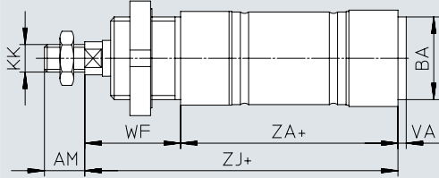
MQ – Short end cap without swivel mounting
