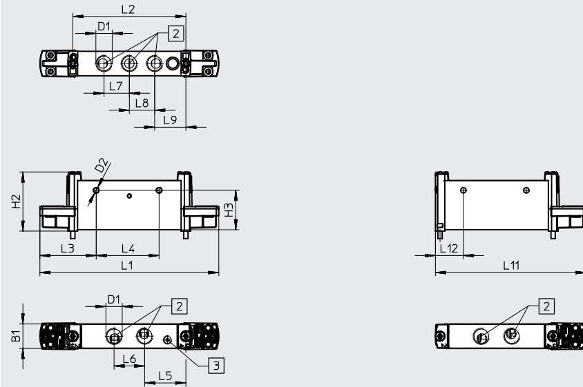
[2] Anschlüsse 1...5
