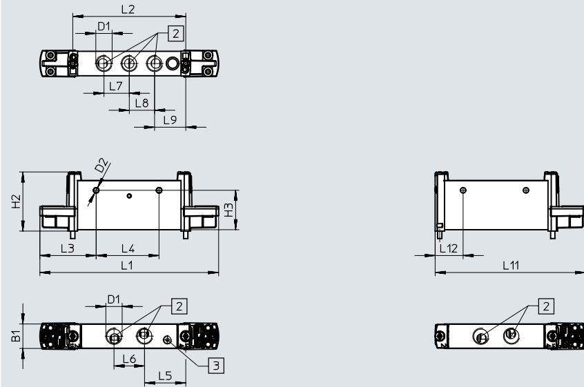
[2] Ports 1...5
