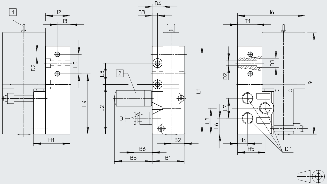
[1] Plug vanes
