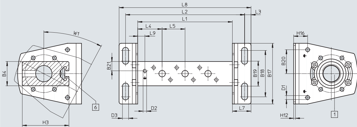
[1] Port 1: G3/4
