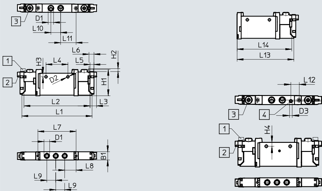
[1] Vertical electrical connection
