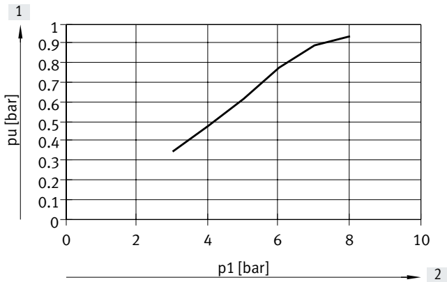
Vacuum as a function of operating pressure
