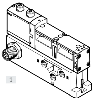
[1] 1xM12 plug, 4-pin to EN 61076-2-101
