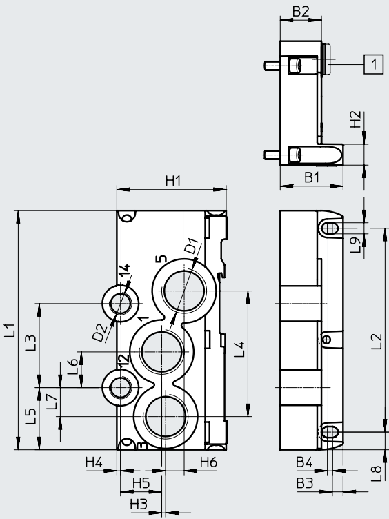
[1] Blanking plug
