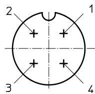
[1] 1xM12 plug, 4-pin to EN 61076-2-101
