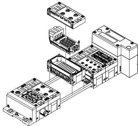
CPX terminal in metal design
