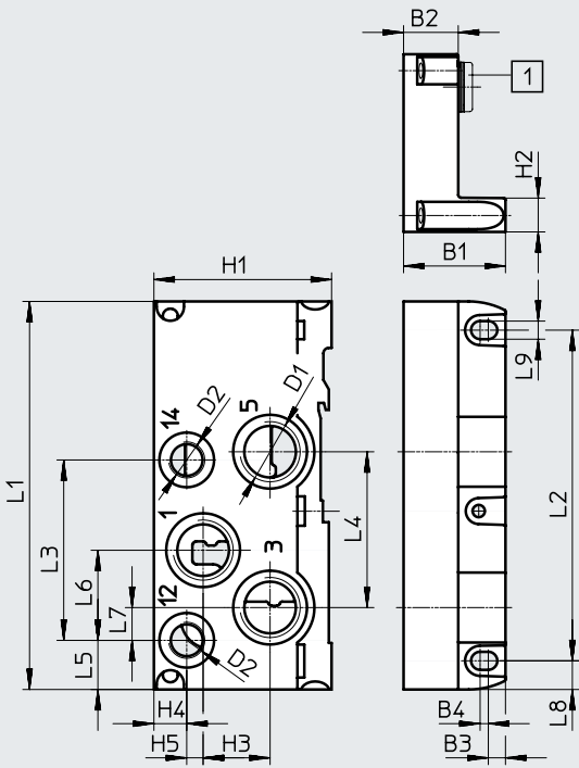
[1] Blanking plug
