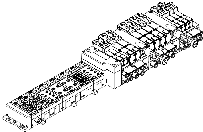
VTSA/VTSA-F with electrical peripherals CPX
