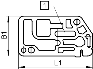
[1] With elongated hole, internal pilot air supply
