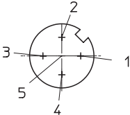
[1] 1xM12 plug, 5-pin
