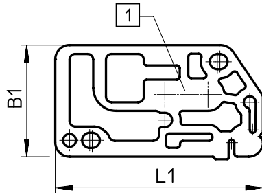
[1] Without elongated hole, external pilot air supply
