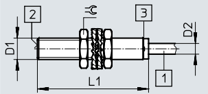
M12 – Flush fitting Cable
