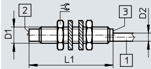
M12 – Partially flush fitting Cable
