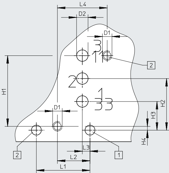
[1] Hole for coding pin, 1.7 +0.2 mm deep [2] Mounting thread, 4.6 +1 mm deep
