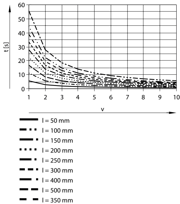
Positioning time t as a function of speed level v and stroke l with axial kit for EPCS-BS-60-5P
