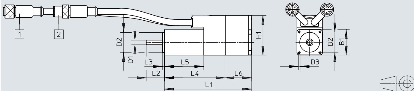
Dimensions – Stepper motors EMMS-ST...-SB/SEB, size 28
