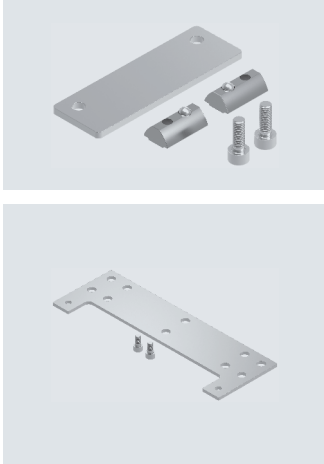
[1] Switch lug DASI-...-SL [2] Sensor bracket DASI-...-SR Inductive proximity switches → page 28
