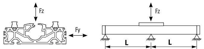
Force F_z
