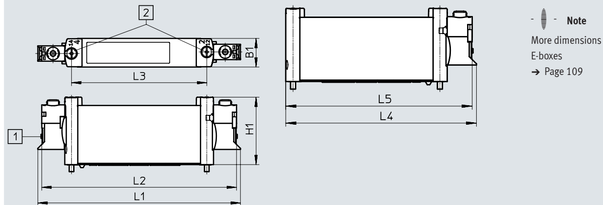
[1] Horizontal electrical connection [2] Manual override
