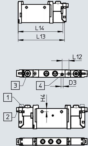
[1] Vertical electrical connection [2] Horizontal electrical connection [3] Manual override [4] Port for external pilot air supply
