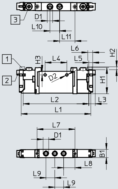
[1] Vertical electrical connection [2] Horizontal electrical connection [3] Manual override [4] Port for external pilot air supply
