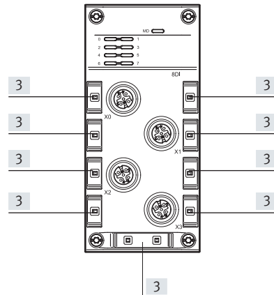
[1] Electrical connection, inputs [2] LED indicators [3] Space for inscription label
