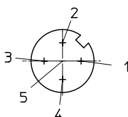
[1] Conector M12x1, pasador, 5 pines
