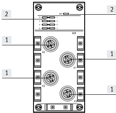
[1] Electrical connection, inputs [2] LED indicators [3] Space for inscription label
