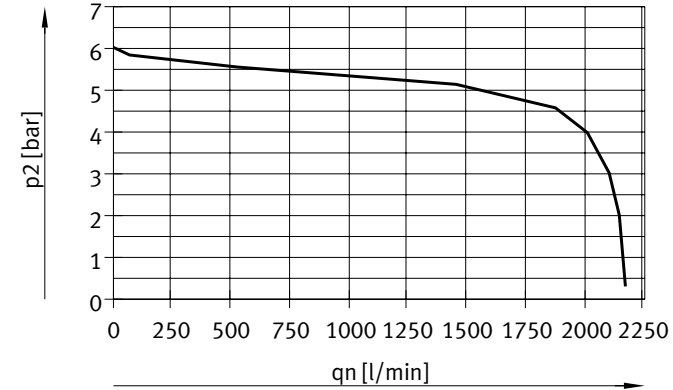
Input pressure 10 bar, set regulated pressure 6 bar
