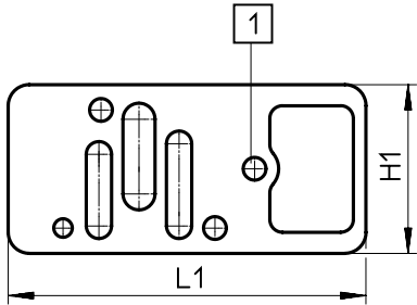
[1] With hole, internal pilot air supply
