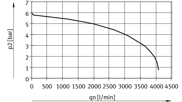
Input pressure 10 bar, set regulated pressure 6 bar
