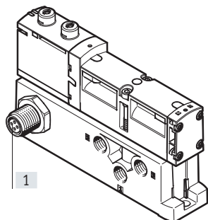
[1] Plug M12x1, 4-pin to EN 61076-2-101
