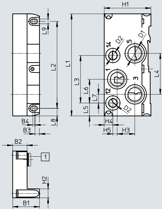
Right-hand end plate, VABE-S6-1R...
