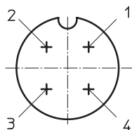
[1] Plug M12x1, 4-pin to EN 61076-2-101
