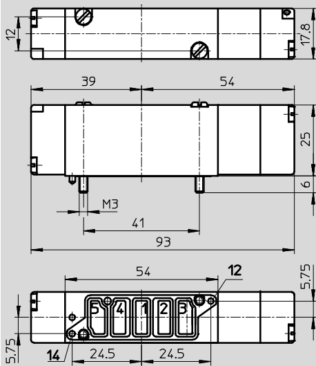
Sub-base valve
