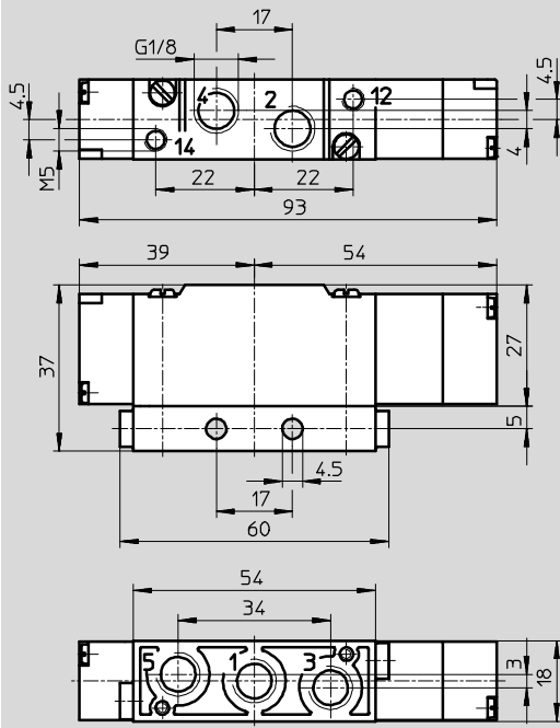
Semi in-line valve with thread G1/8
