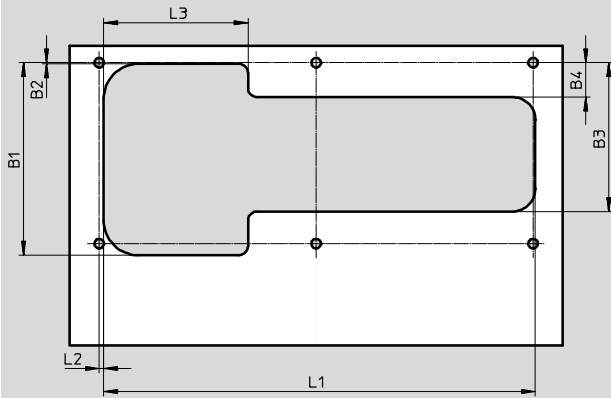
Dimensions – Recess for control cabinet installation, outlet direction underneath, size 18
