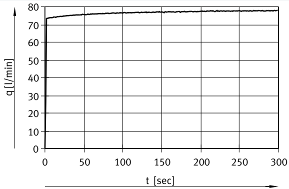
Flow rate q_n as a function of switch-on point at 300 V and an operating pressure of 5 bar
