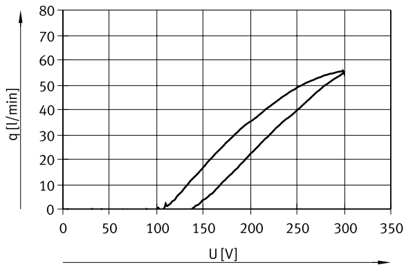
Flow rate q_n as a function of switch-on point at 300 V and an operating pressure of 3 bar
