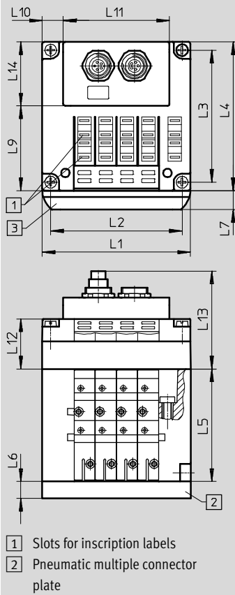
Valve terminal with installation system CPI – CPV10/14
