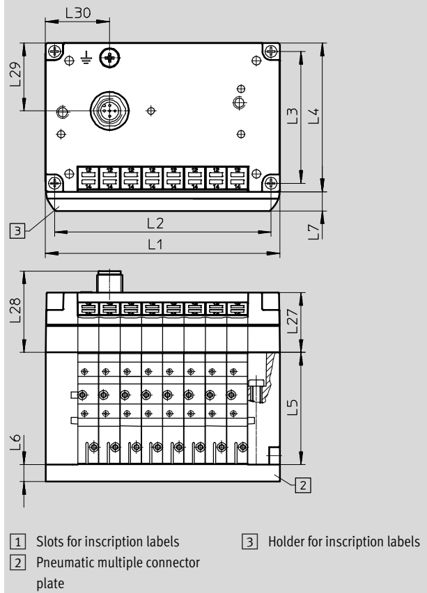
Valve terminal with I-Port interface/IO-Link – CPV10/14
