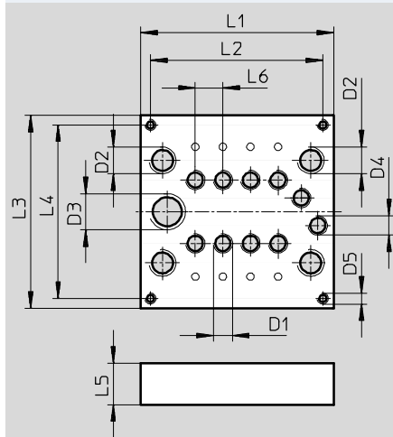
Pneumatic multiple connector plate – CPV10/14/18
