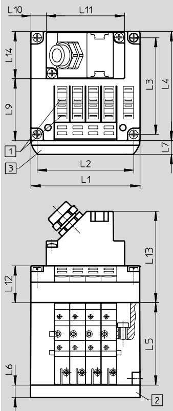
Valve terminal with multi-pin plug connection – CPV10/14/18
