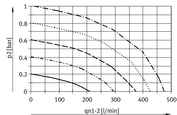
Flow rate q_n from 1 > 2 as a function of output pressure p_2 1 bar Flow rate q_n from 2 > 3 as a function of output pressure p_2 1 bar
