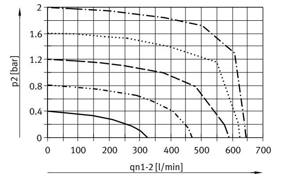
Flow rate q_n from 1 > 2 as a function of output pressure p_2 2 bar Flow rate q_n from 2 > 3 as a function of output pressure p_2 2 bar
