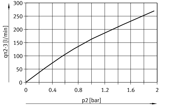
Flow rate q_n from 1 > 2 as a function of output pressure p_2 2 bar Flow rate q_n from 2 > 3 as a function of output pressure p_2 2 bar
