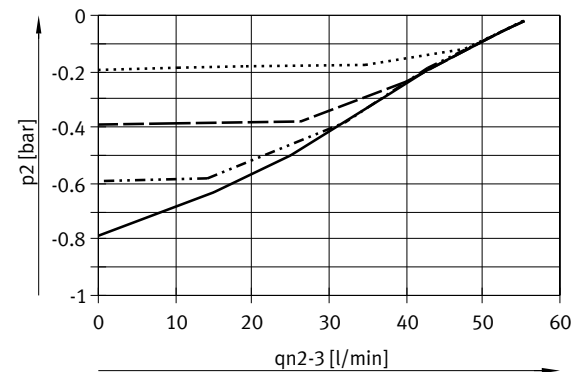
Flow rate q_n from 1 > 2 as a function of output pressure p_2 \pm 1 bar Flow rate q_n from 2 > 3 as a function of output pressure p_2 \pm 1 bar
