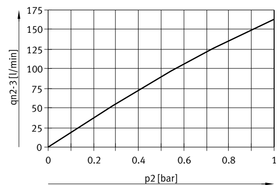
Flow rate q_n from 1 > 2 as a function of output pressure p_2 1 bar Flow rate q_n from 2 > 3 as a function of output pressure p_2 1 bar
