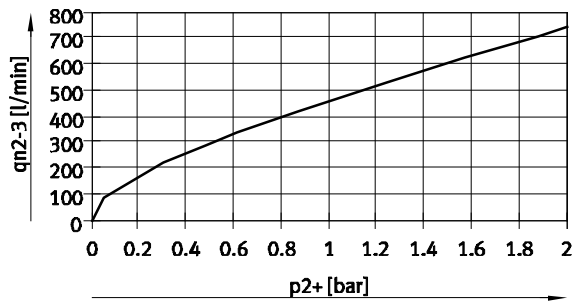
VPPM-8TA-...-0L10H-... (10 bar)
