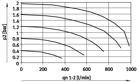
VPPM-8TA-...-0L2H-... (2 bar)
