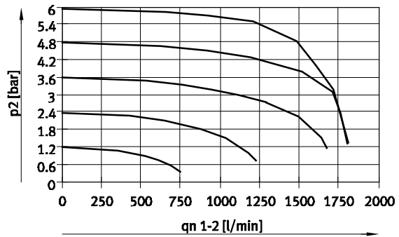
VPPM-8TA-...-0L6H-... (6 bar)
