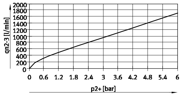
VPPM-8TA-...-0L6H-... (6 bar)
