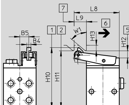
Toggle lever valve LS-4-1/8
