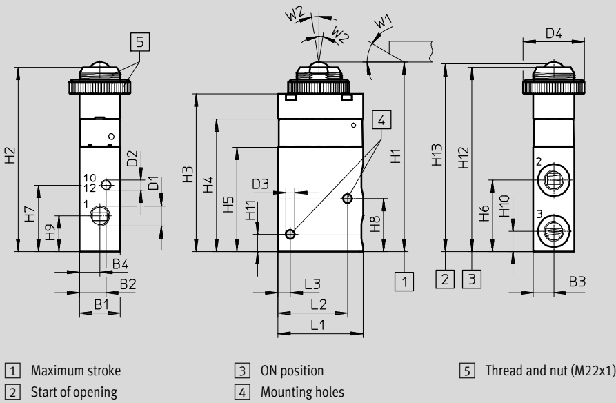
Ball actuated valve VMEM-BTC...32...G18
