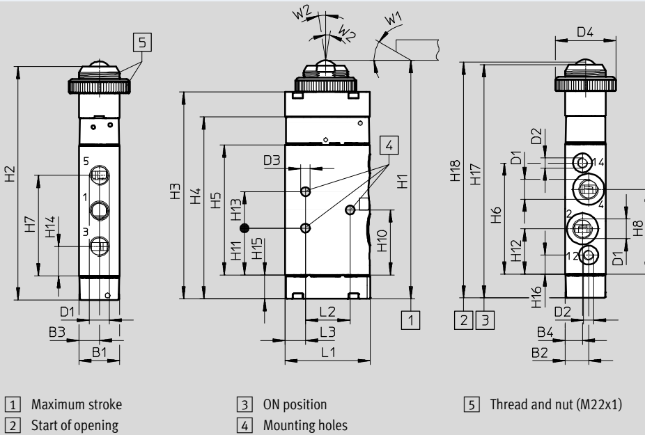
Ball actuated valve VMEM-BC/BCZ...52...G18
