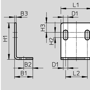
Mounting bracket HV-1/8
