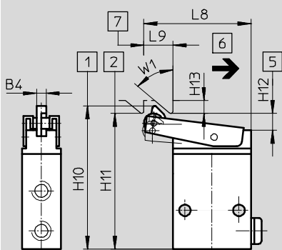
Toggle lever valve LS-3-1/8, LOS-3-1/8
