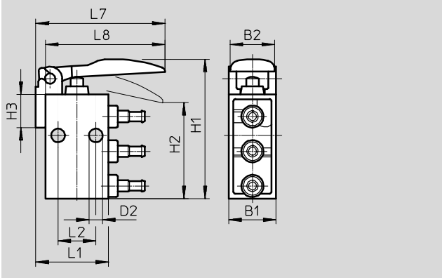
Finger lever valve TH/O-3-PK-3
