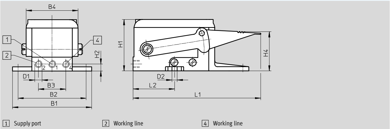
Foot valve with detent FP-5-1/4-B
