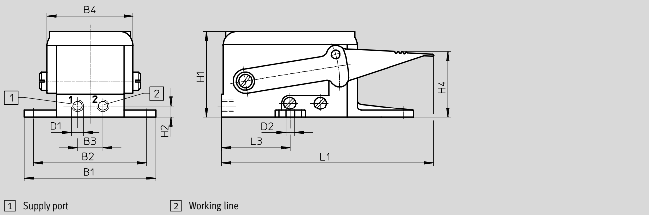
Foot valve with detent FP-3-1/4-B
