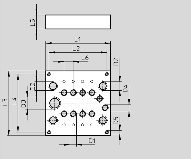
Multiple connector plate
