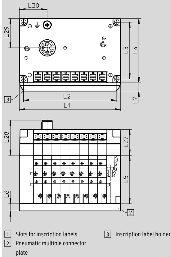
Valve terminal with I-Port interface/IO-Link – CPV10/14
