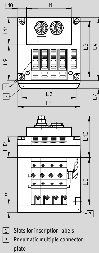
Valve terminal with installation system CPI – CPV10/14/18
