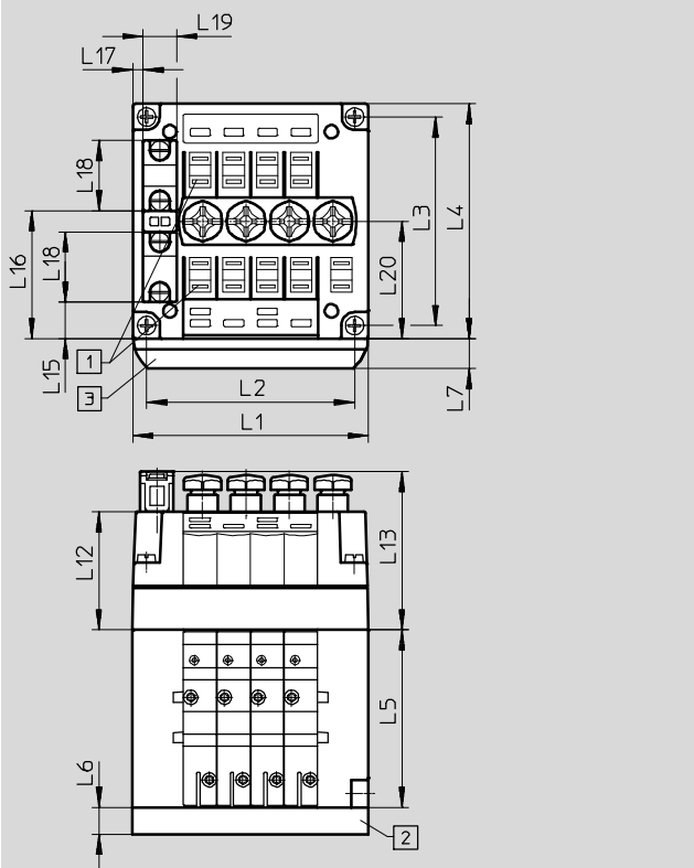
Valve terminal with AS-Interface connection and additional inputs – CPV10/14
