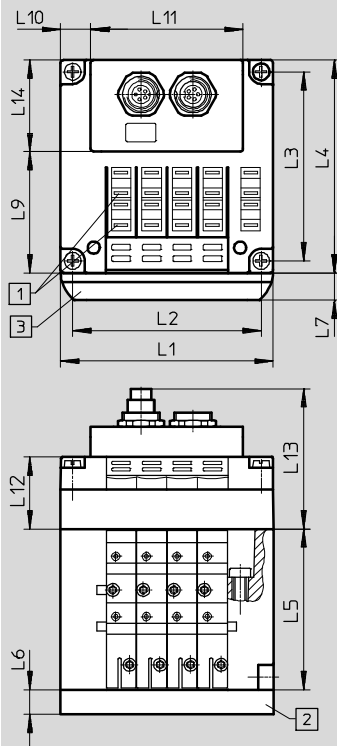
Valve terminal with installation system CPI – CPV10/14/18
