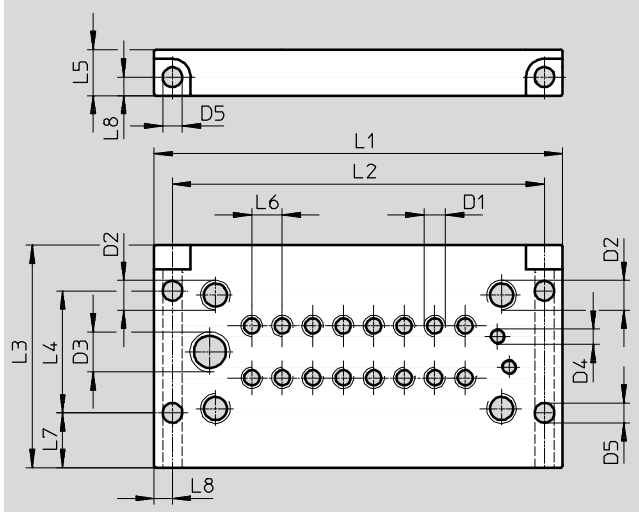
Flanged pneumatic multiple connector plate – CPV10/14/18
