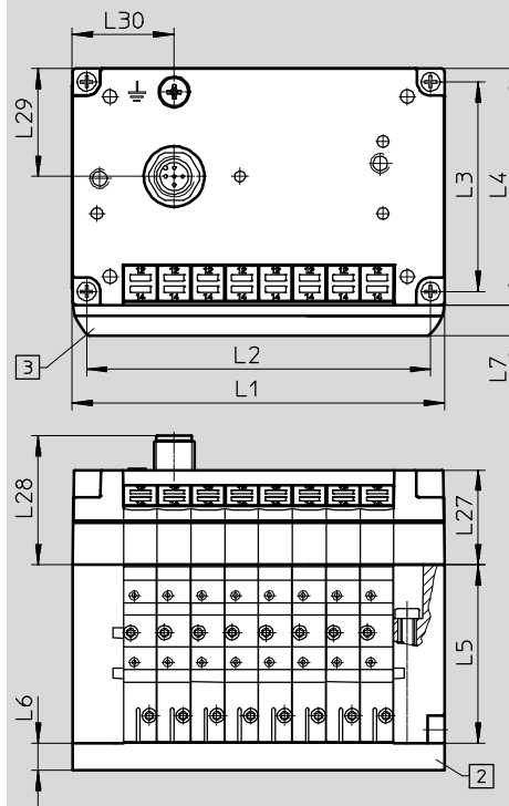
Valve terminal with I-Port interface/IO-Link – CPV10/14
