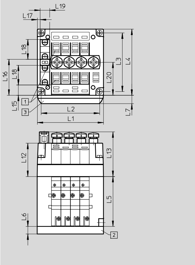
Valve terminal with AS-Interface connection and additional inputs – CPV10/14
