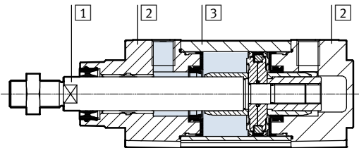
Sectional view – Basic design
