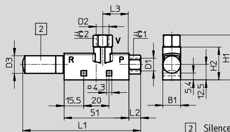
2 Silencer
