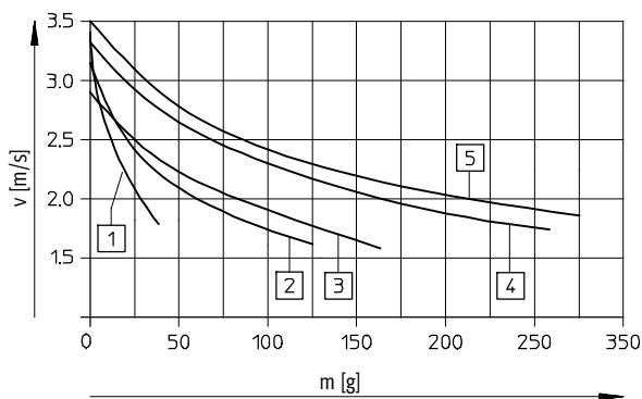
Maximum permissible impact velocity v as a function of the applied load m
