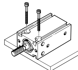
Horizontal mounting
