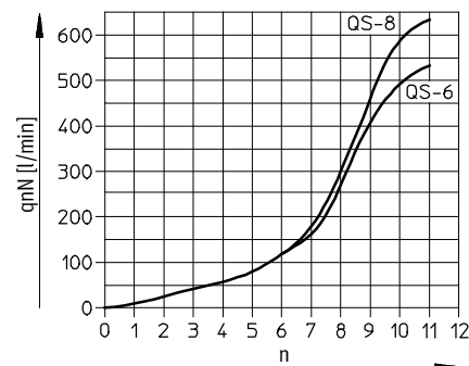
Standard nominal flow rate q_{pN} at 6 → 5 bar as a function of turns of the adjusting screw n
