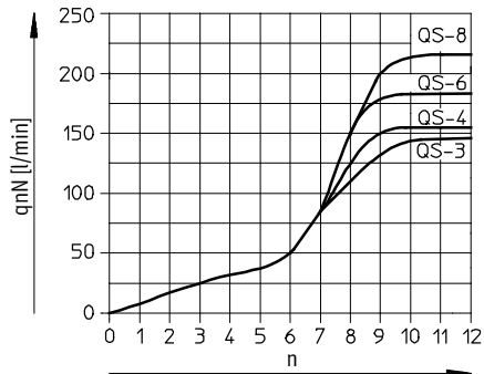
Standard nominal flow rate q_{nN} at 6 → 5 bar as a function of turns of the adjusting screw n GRLA/GRLZ-1/8
