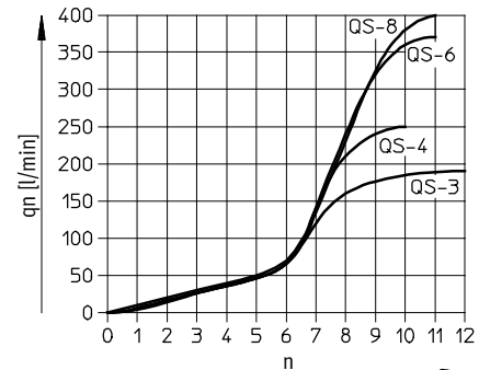
Standard flow rate q_n at 6 → 0 bar as a function of turns of the adjusting screw n GRLA/GRLZ-1/8
