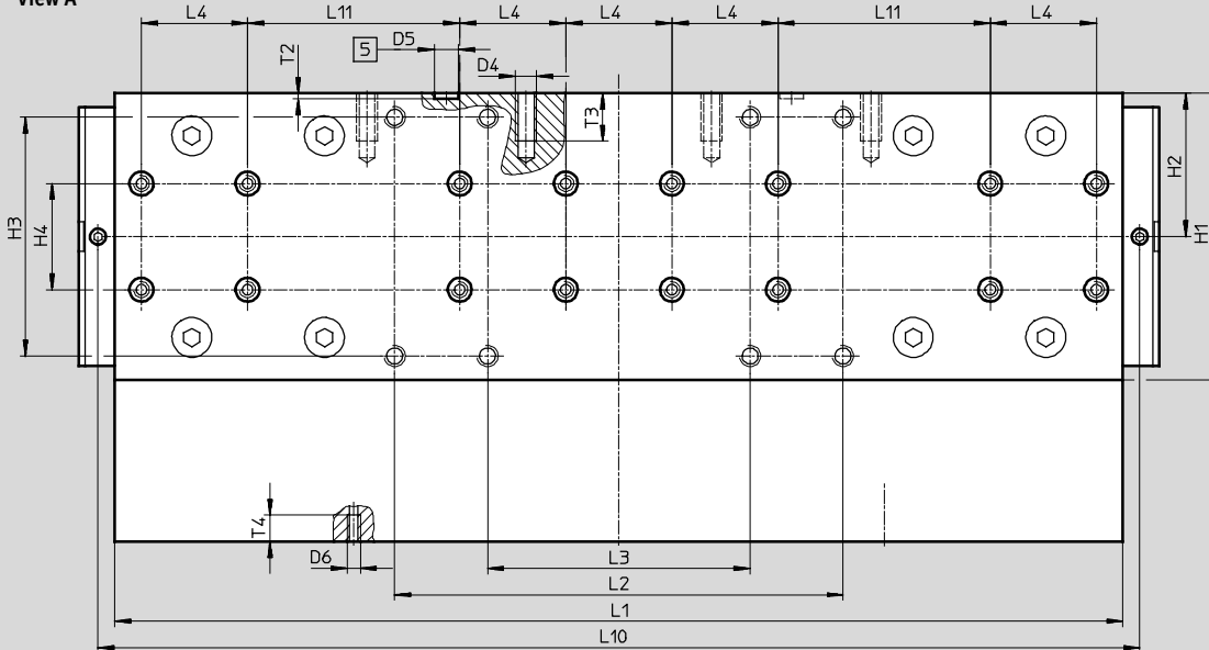
View A
