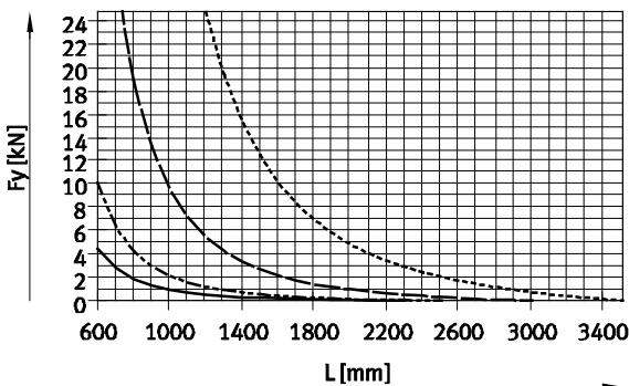
Force F_y
