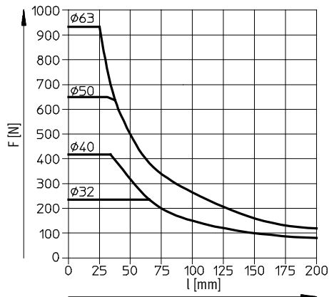
DFM-32 ... 63-KF Stroke 80 ... 100 mm
