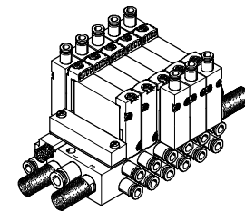
VUWG-B valve manifold consisting of sub-base valves
