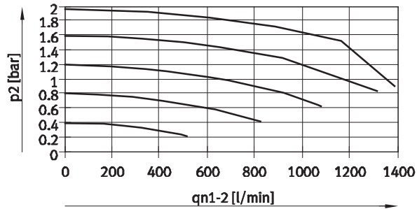
VPPM-8TA-...-0L2H-... (2 bar)
