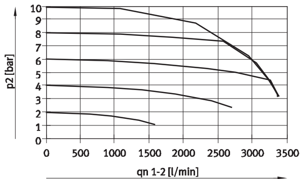
VPPM-8TA-...-0L10H-... (10 bar)
