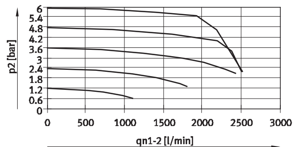
VPPM-8TA-...-0L6H-... (6 bar)
