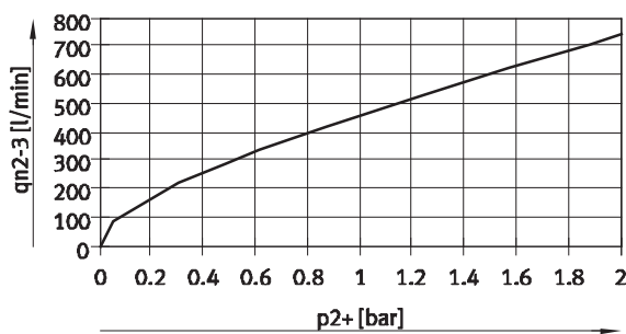
VPPM-8TA-...-0L2H-... (2 bar)
