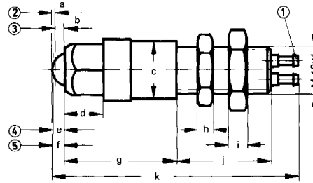
Type SDK-4-PK-3
