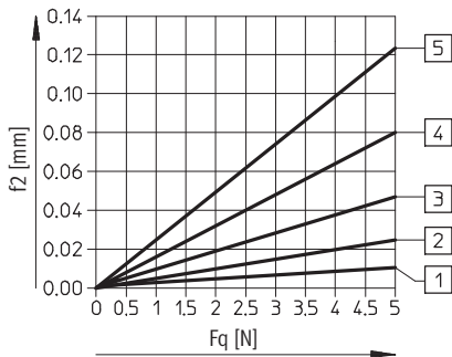
Piston \varnothing 16 mm
