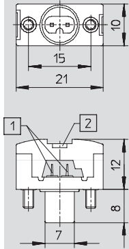
Flat cable socket ASI-SD-FK-M12
