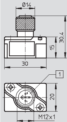
Flat cable socket ASI-SD-FK-M12
