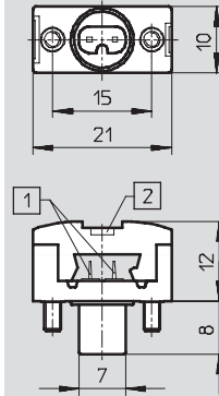
Blanking plug ASI-SD-FK-BL
