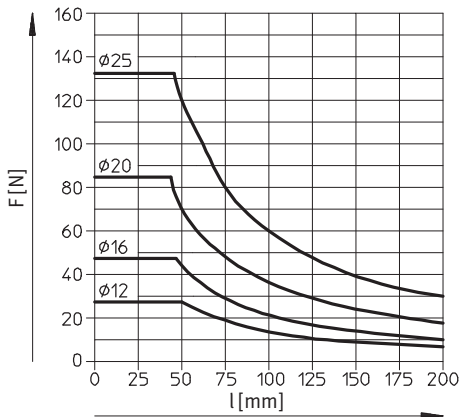
DFM-12 ... 25-GF Hub 30 mm
