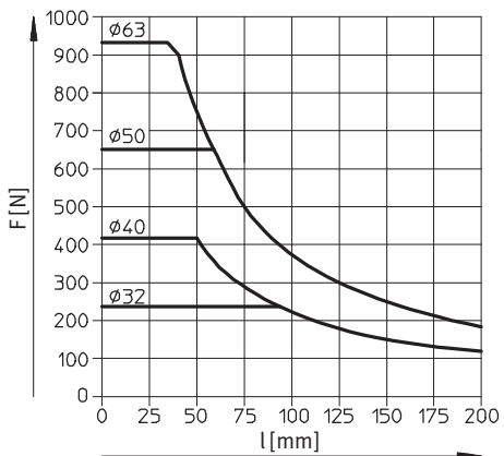
DFM-32 ... 63-GF Hub 50 mm
