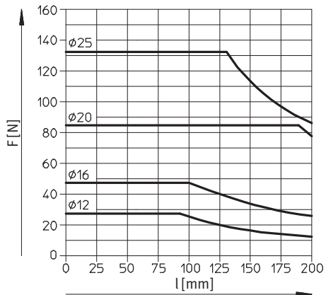
DFM-12 ... 25-GF Hub 40 ... 100 mm
